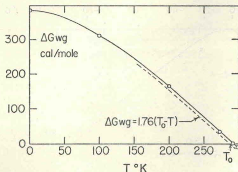
FIG. 6. Gibbs free energy difference of white and gray tin vs temperature. The solid curve is from Bronsted's heat capacity and heat of transformation data. The dashed curve represents adjusted values which give \Delta G_{wg} = 0 at a transition temperature ( T_0 ) of 286.4°K.
