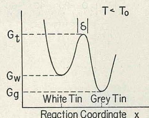
FIG. 5. Free energy of tin atom vs distance along the transformation path.
